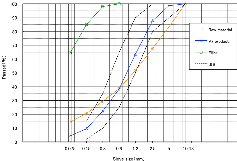
Grading curves
