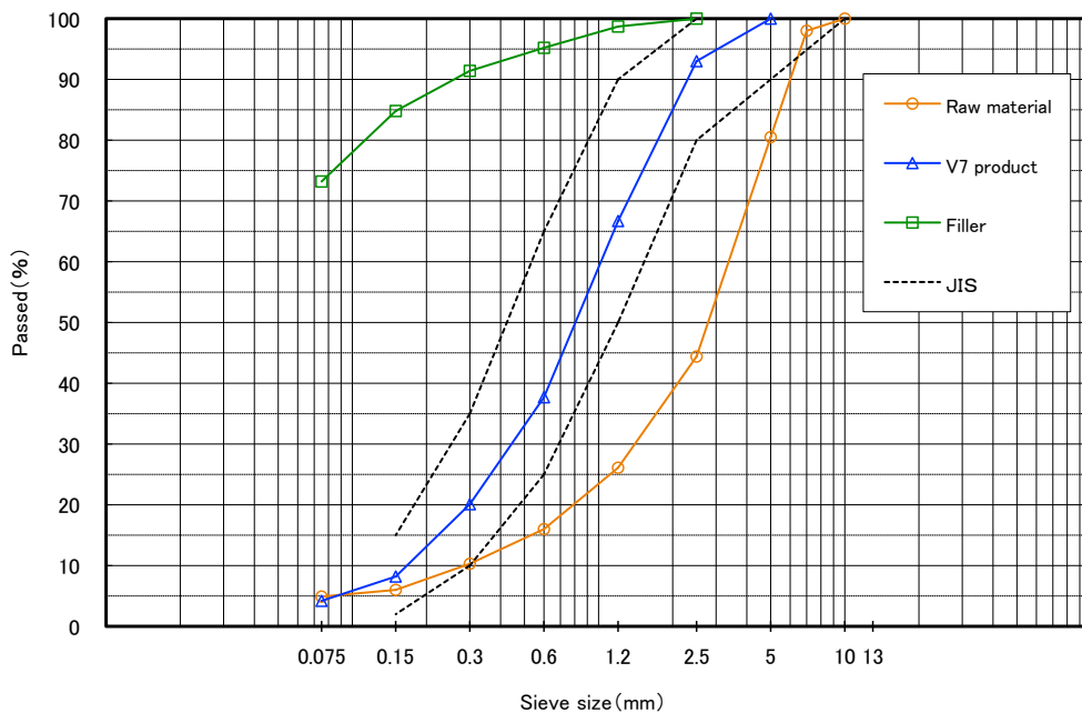
Grading curves
