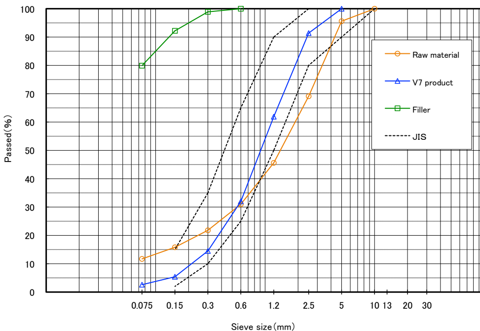
Grading curves
